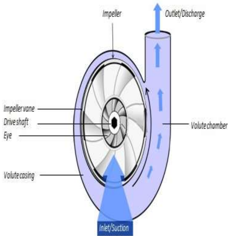
Figure 2. Volute case design
